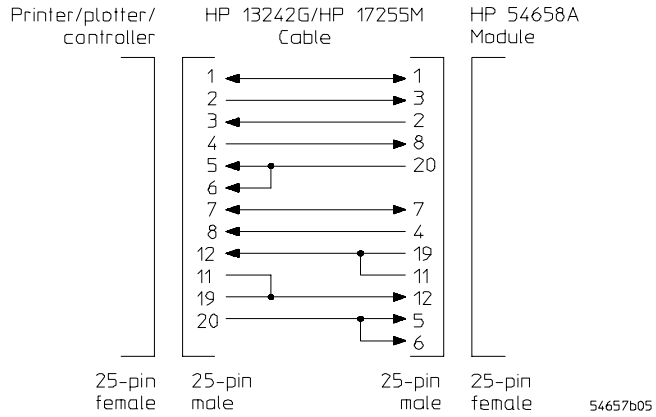
Pin out of HP 13242G/HP 17255M RS-232 cable
