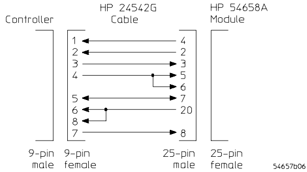
Pin out of HP 24542G RS-232 cable
