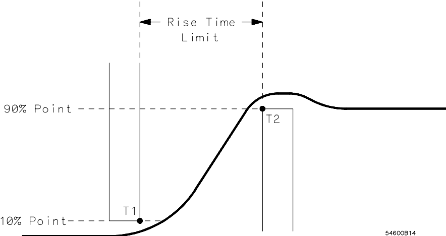
Example of a definition of a rise time testing mask
