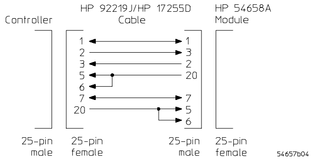
Pin out of HP 92219J/ HP 17255D RS-232 cable
